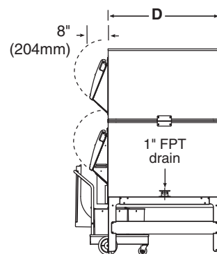
Models DEV3200, 3900, 4600
