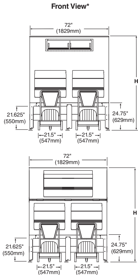
Models DEV3200, 3900, 4600
