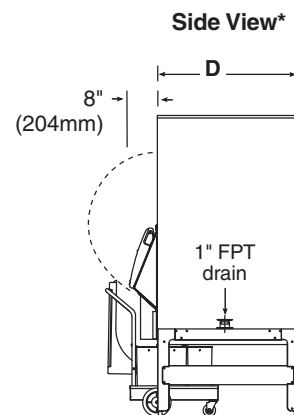
Models DEV2100, 2250, 2650
