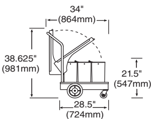
Models DEV3200, 3900, 4600
