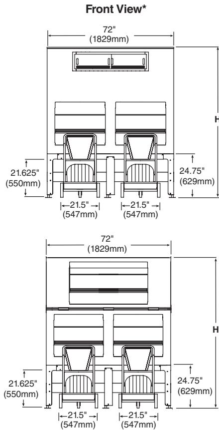
Models DEV3200, 3900, 4600
