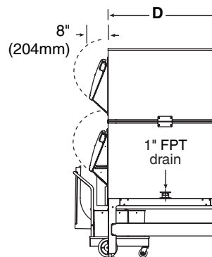
Models DEV3200, 3900, 4600
