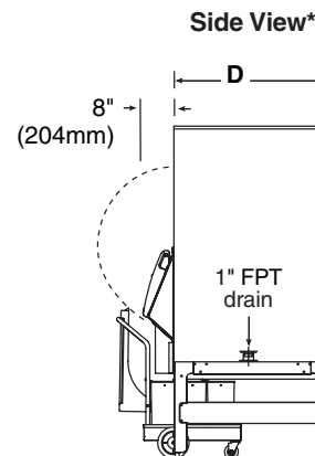
Models DEV2100, 2250, 2650
