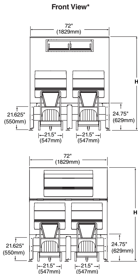
Models DEV3200, 3900, 4600
