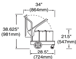
Models DEV3200, 3900, 4600
